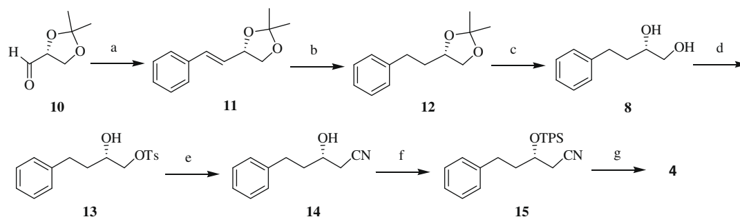
Scheme 2. Reagents and conditions: (a) [PhCH_2Ph_3]Br , n-BuLi , THF, 0 °C, 0.5 h, 90%, E/Z = 80:20 ; (b) H_2 , 10% Pd/C, MeOH, rt, 6 h, 96%; (c) 2 M HCl, MeOH, rt, 1 h, 95%; (d) TsCl, (C_2H_5)_3N , (n-Bu)_2SnO , 0 °C–rt, 4 h, 76%; (e) KCN, Ethanol/ H_2O (3:2), rt, 10 h, 90%; (f) TBDPS-Cl, imidazole, anhydrous CH_2Cl_2 , rt, 3 h, 96%; (g) DIBAL-H, anhydrous CH_2Cl_2 , –78 °C, 0.5 h, 72%.
