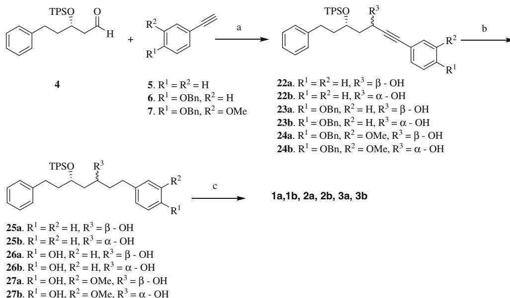
Scheme 4. Reagents and conditions: (a) n -BuLi, THF, 0 °C–rt, 2 h, 90%; (b) 10% Pd/C, MeOH, rt, 8 h, 95%; (c) PTSA, MeOH, rt, 1 h, 95%.
