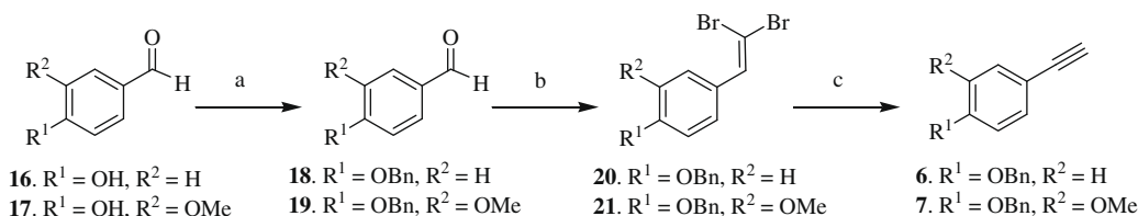
Scheme 3. Reagents and conditions: (a) BnBr , K_2CO_3 , Acetone, 0 °C–rt, 95%; (b) PPh_3 , CBr_4 , CH_2Cl_2 , 0 °C, 0.5 h, 90%; (c) EtMgBr , THF, 0 °C–rt, 0.5 h, 95%.
